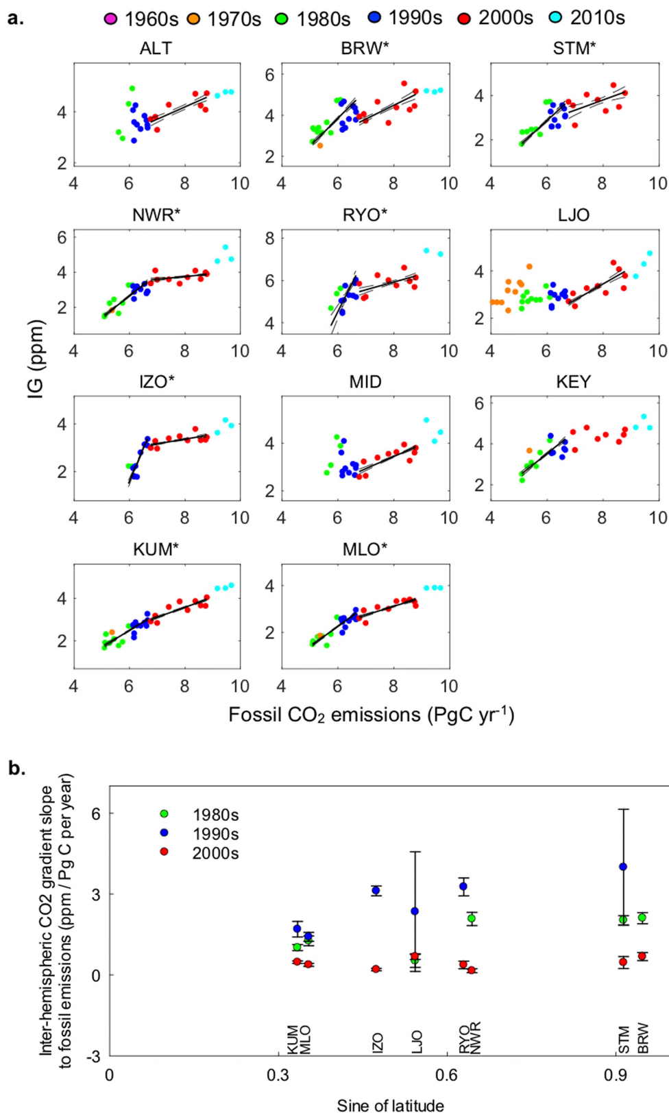
Extended Data Fig. 2 | Interhemispheric CO 2 gradient plotted against fossil-fuel CO 2 emissions for each decade from the 1960s to the 2010s, and IG-F slopes in the 1980s, 1990s and 2000s. a, Scatter plots of the interhemispheric gradient plotted against emissions from fossil fuels and cement, obtained from CDIAC, for different Northern Hemisphere long-term monitoring stations with sufficient data coverage (see Methods). The SPO station is always taken as the reference from which to calculate the interhemispheric gradient from each station. A station is marked by an asterisk if the correlation coefficient ( r^2 ) between interhemispheric
